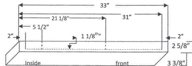
Skid for 3 HP engine
