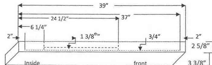
Skid for 3 HP engine
